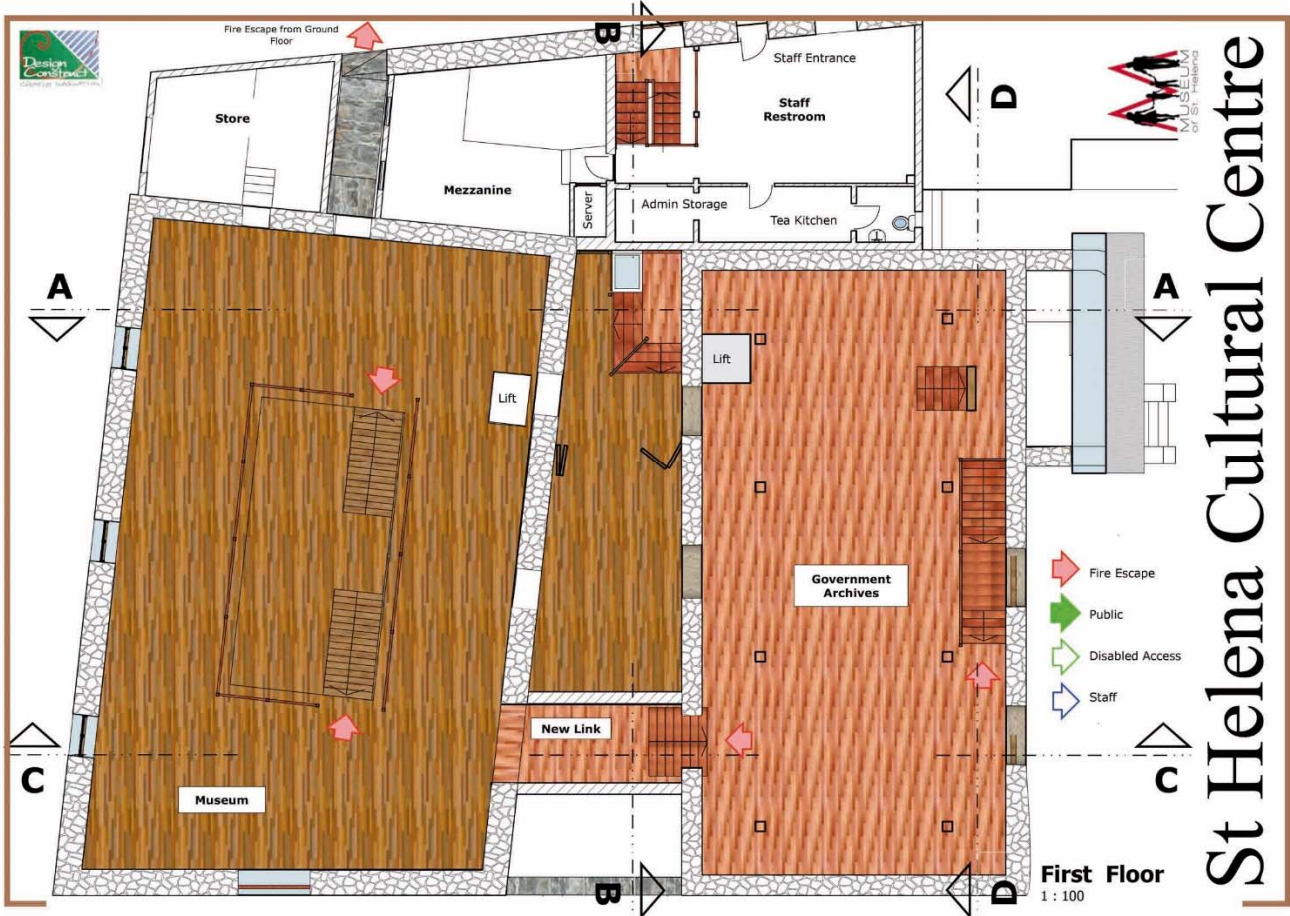
c) First floor view
